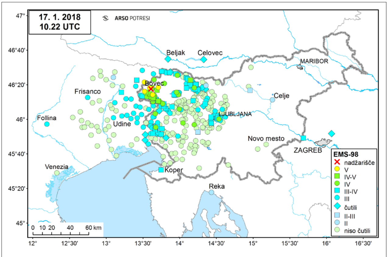
Slika 6: Intenziteta potresa magnitude 3,5 pri Bovcu 17. januarja 2018 ob 10:22 po UTC v posameznih naseljih Figure 6: Intensity of the earthquake near Bovec ( M_{LV}=3.5 ) on 17 January 2018 at 10:22 UTC in individual settlements. Nadžarišče = epicentre; čutili = felt; niso čutili = not felt
