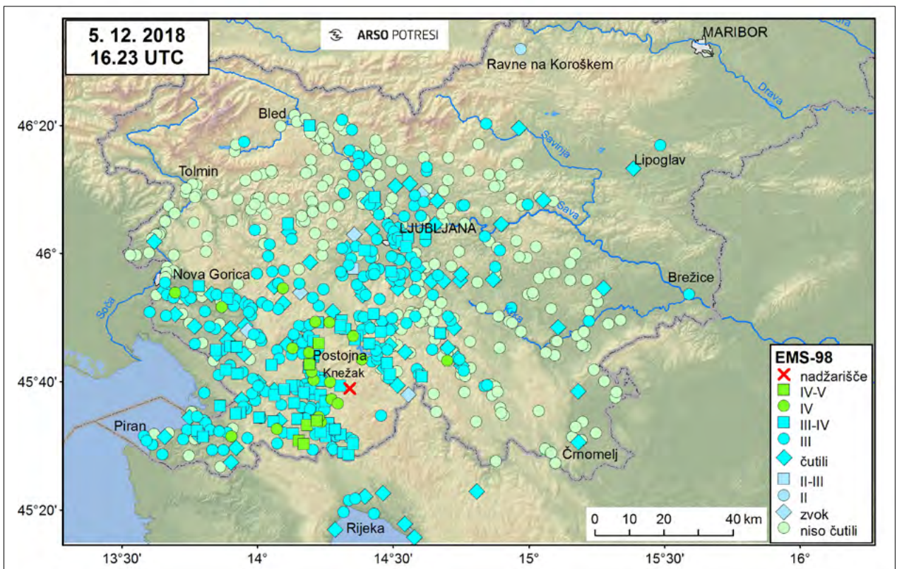
Slika 7: Intenziteta potresa magnitude 3,4 pri Knežaku 5. decembra 2018 ob 16:23 po UTC v posameznih naseljih Figure 7: Intensity of the earthquake near Knežak ( M_{LV}=3.4 ) on 5 December 2018 at 16:23 UTC in individual settlements. Nadžarišče = epicentre; čutili = felt; zvok = thunder; niso čutili = not felt
